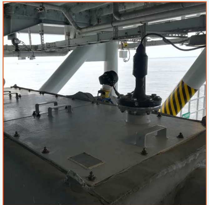
Offshore substation – THE NETHERLANDS Oil separator 3 l/s
